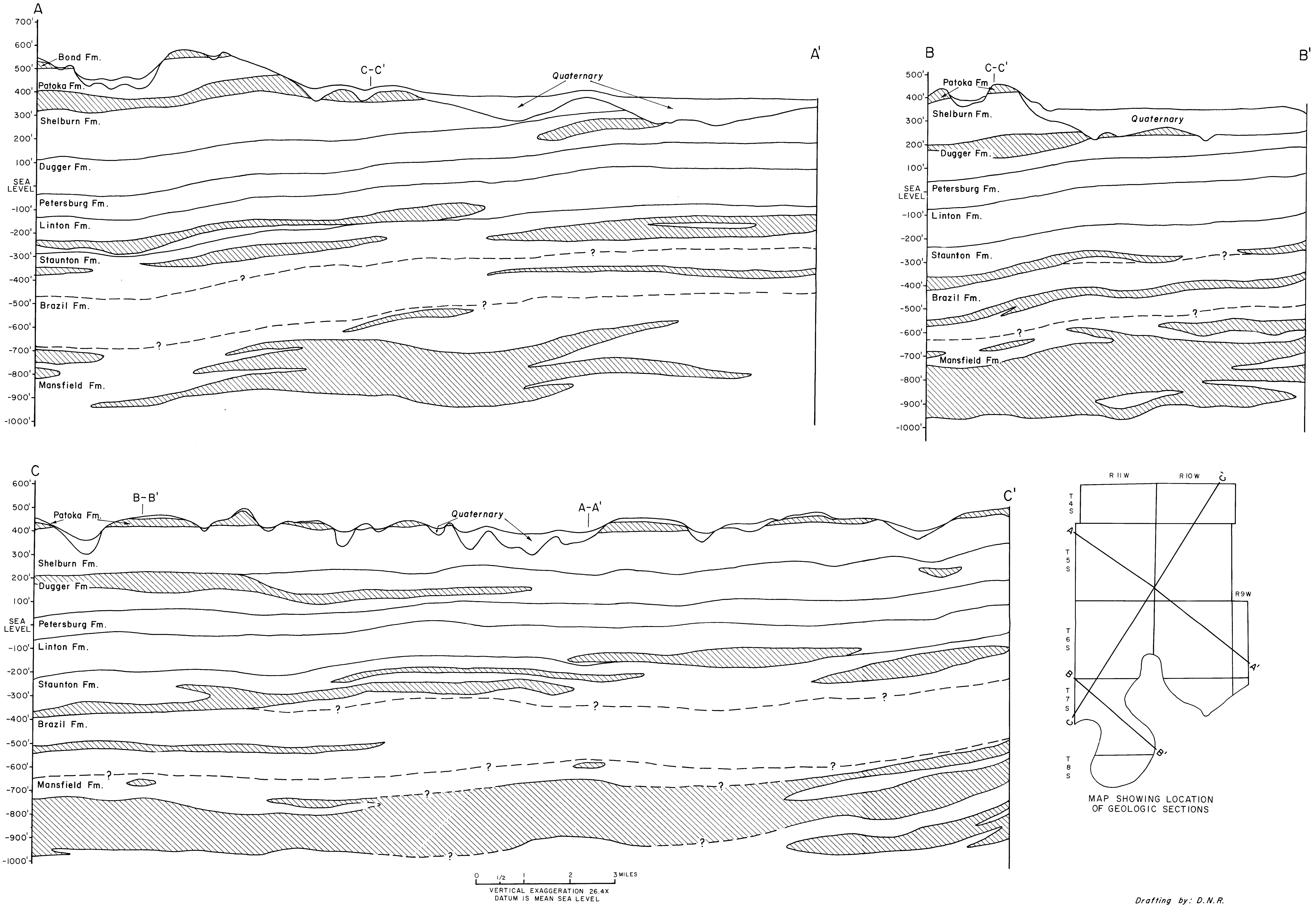
GEOLOGIC SECTIONS OF THE PENNSYLVANIAN SYSTEM WITH PATTERNED AREAS SHOWING THE POSITION OF THE PRINCIPAL SANDSTONE BODIES.
