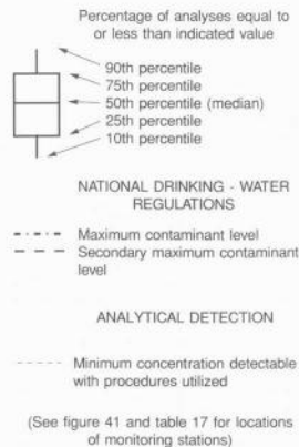
Figure 45. Statistical summary of selected water-quality constituents for selected stream monitoring stations.
