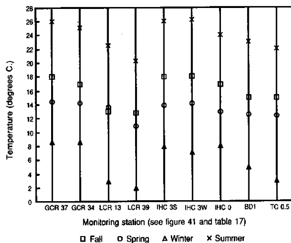
Figure 43. Seasonal median temperature at selected stations
