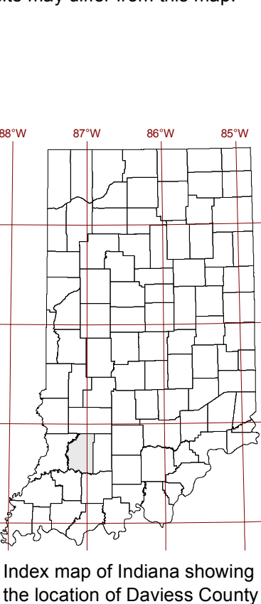
Index map of Indiana showing the location of Daviess County
