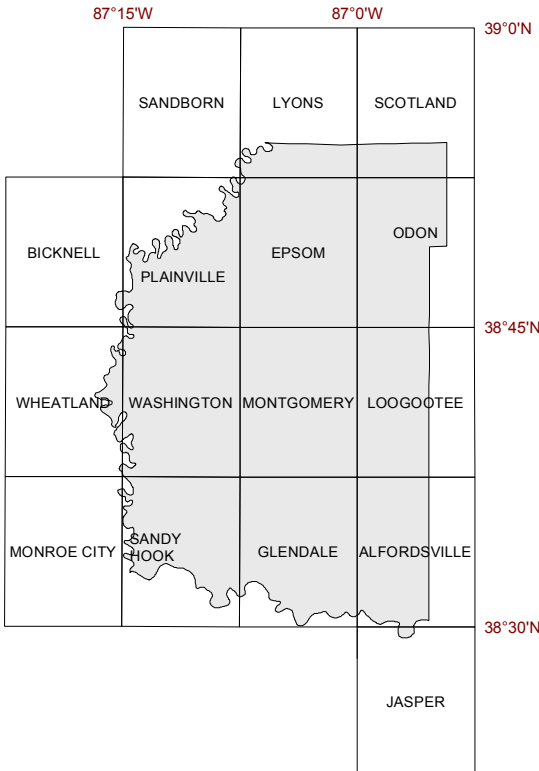
Index map of Daviess County showing U.S. Geological Survey 7 1/2-minute topographic quadrangle map names
