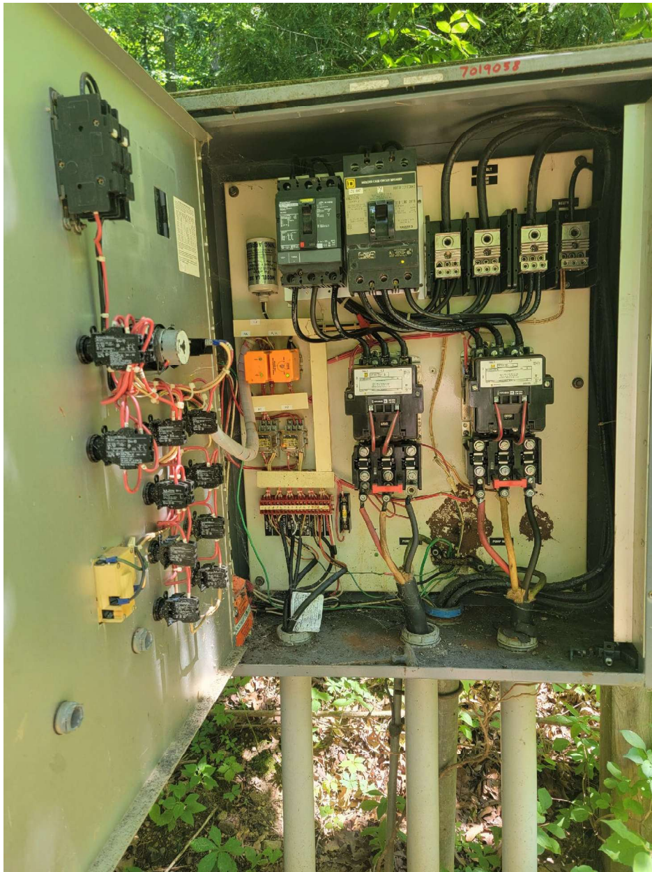
Photograph No. 2 – Sunset Point Lift Station – Base Bid
