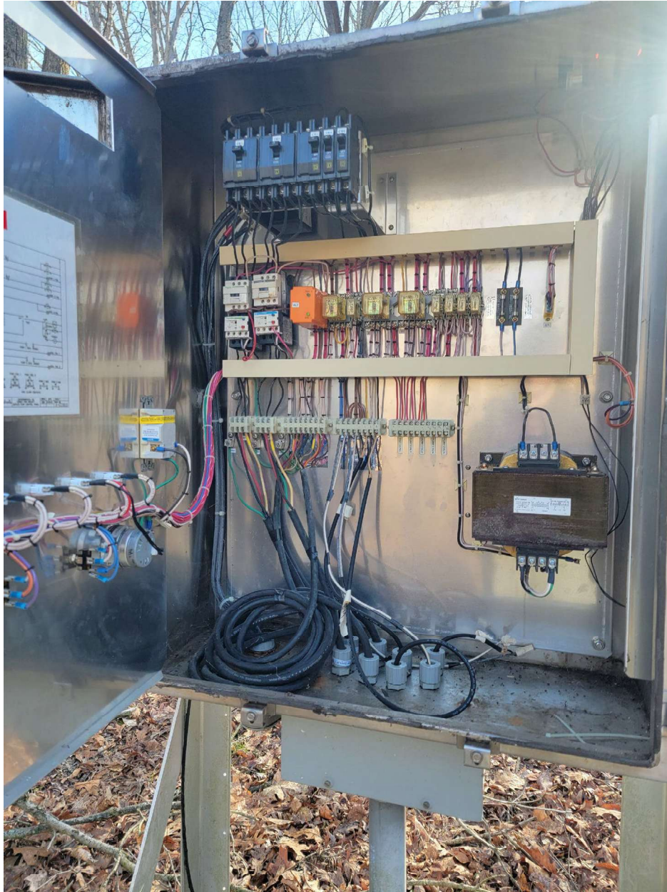
Photograph No. 9 – Newby Gulch Lift Station – Alternate #2
