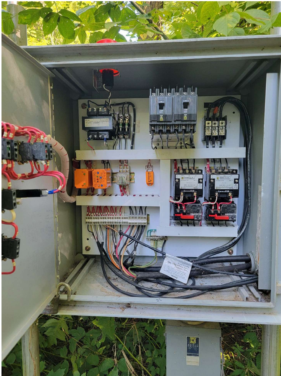
Photograph No. 6 – West Campground Lift Station – Alternate #1
