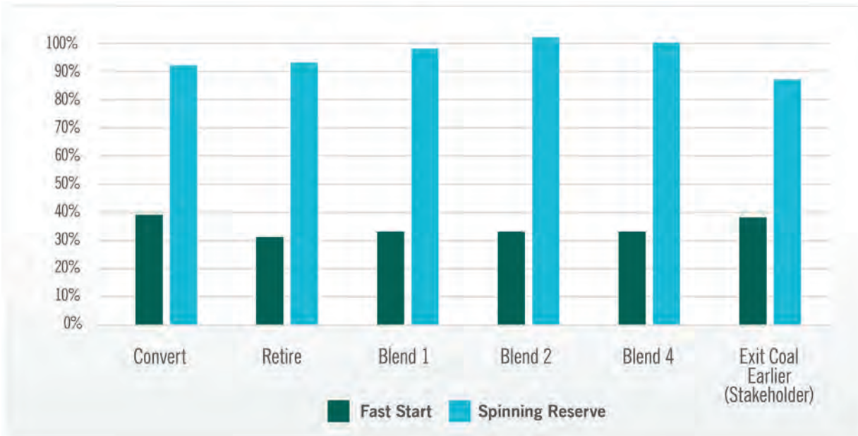
Figure 4-20: Fast Start Capability and Spinning Reserve (%) in 2035
