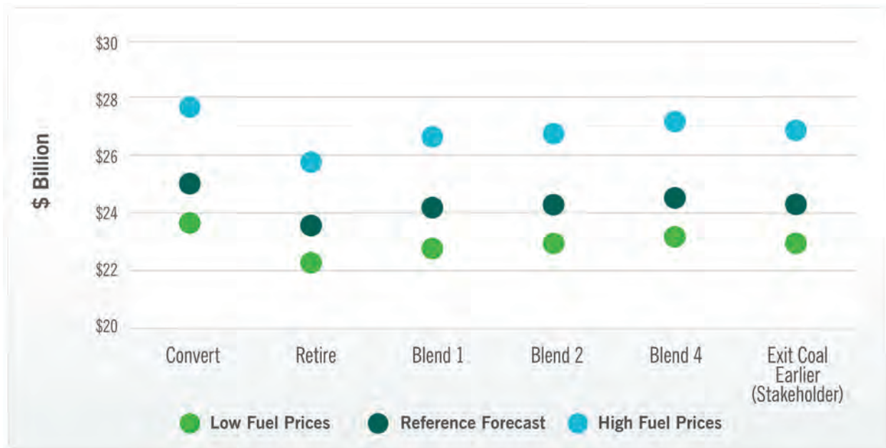
Figure 4-25: PVRR Results for Alternate Fuel Price Forecasts ($B)
