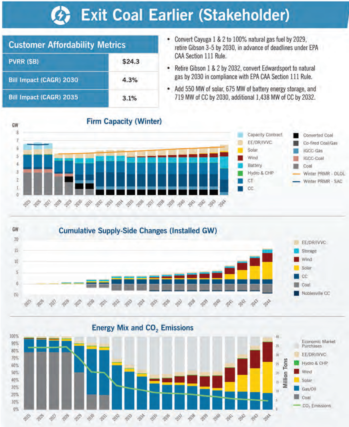
Figure 4-13: Exit Coal Earlier (Stakeholder) Generation Strategy Summary
