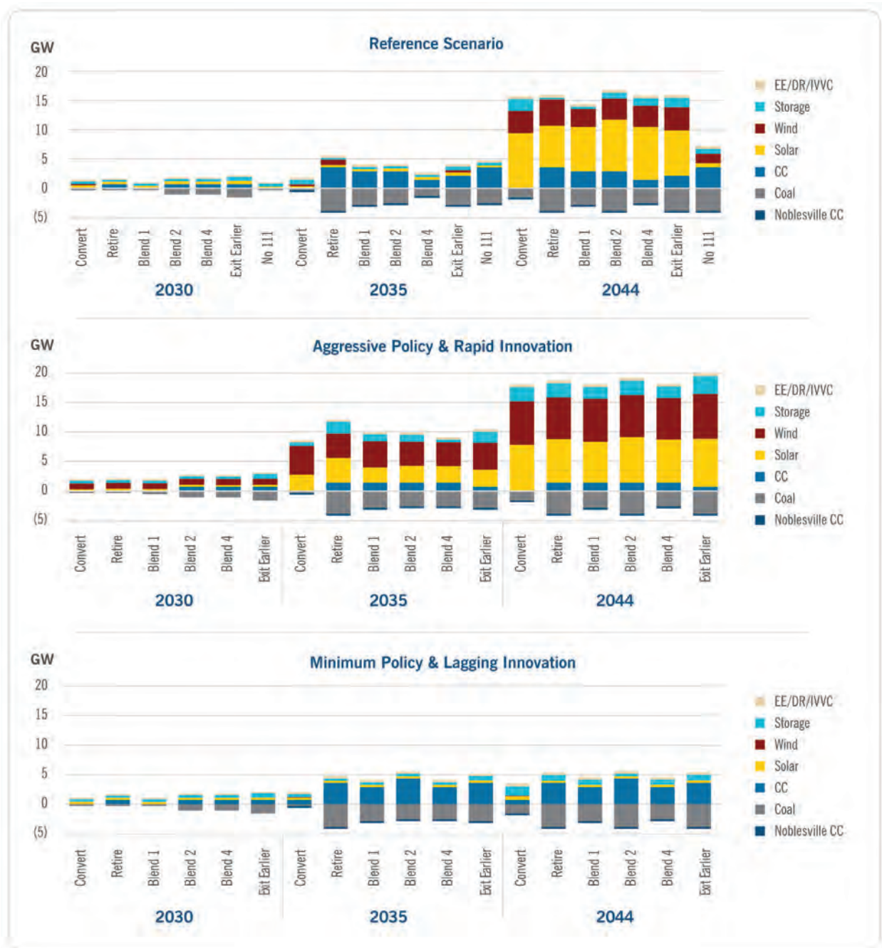
Figure 4-5: Cumulative Resource Additions and Retirements (Installed GW, Beginning-of-Year Basis)
