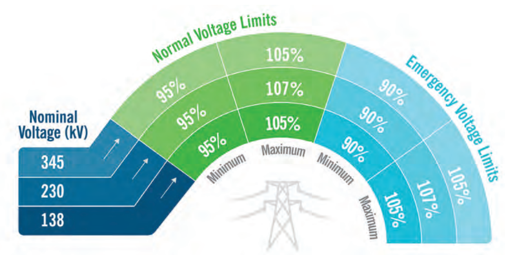
Figure I-1: Transmission System Voltage Limits
