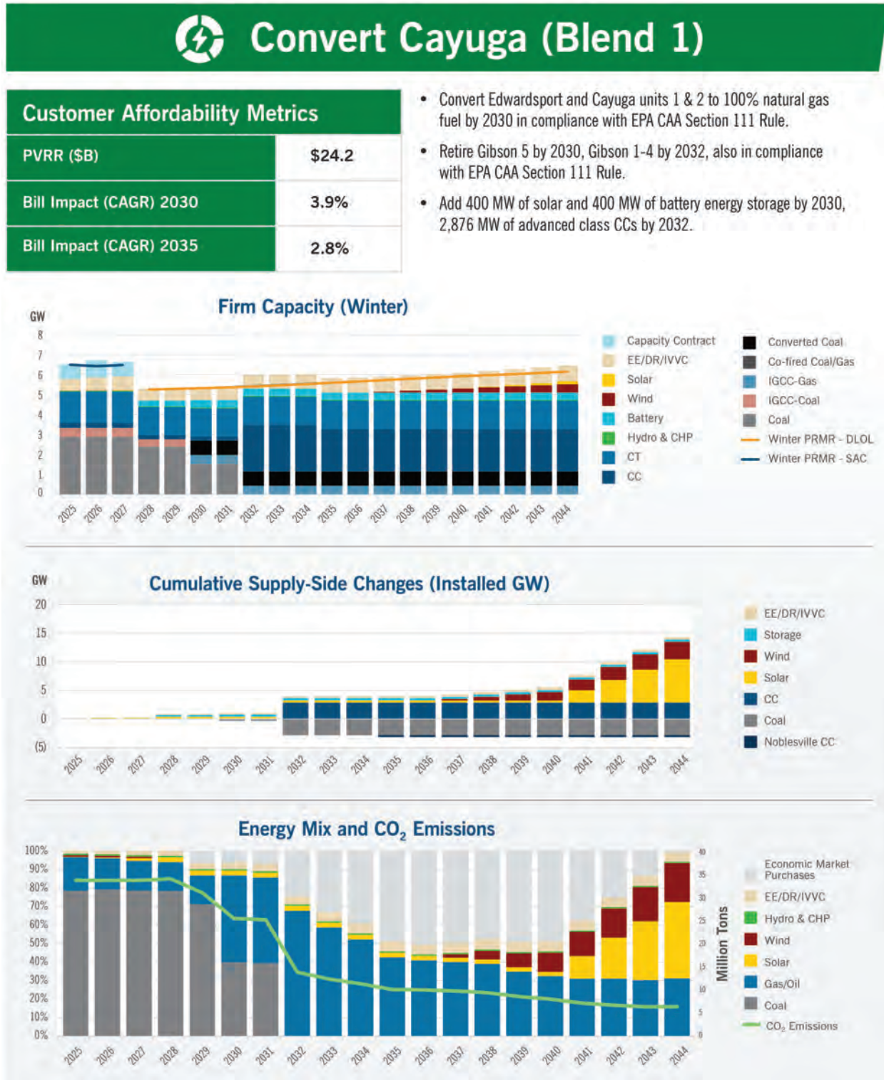
Figure 4-10: Convert Cayuga (Blend 1) Generation Strategy Summary
