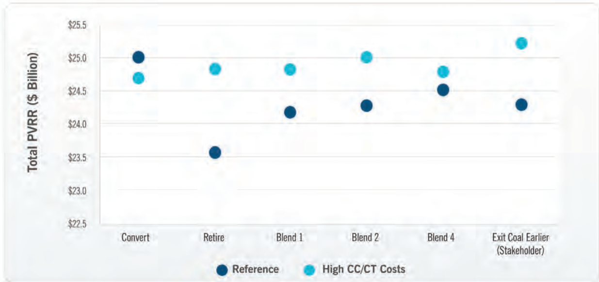
Figure C-23: PVRR Through 2044 for High CC and CT Cost Sensitivity
