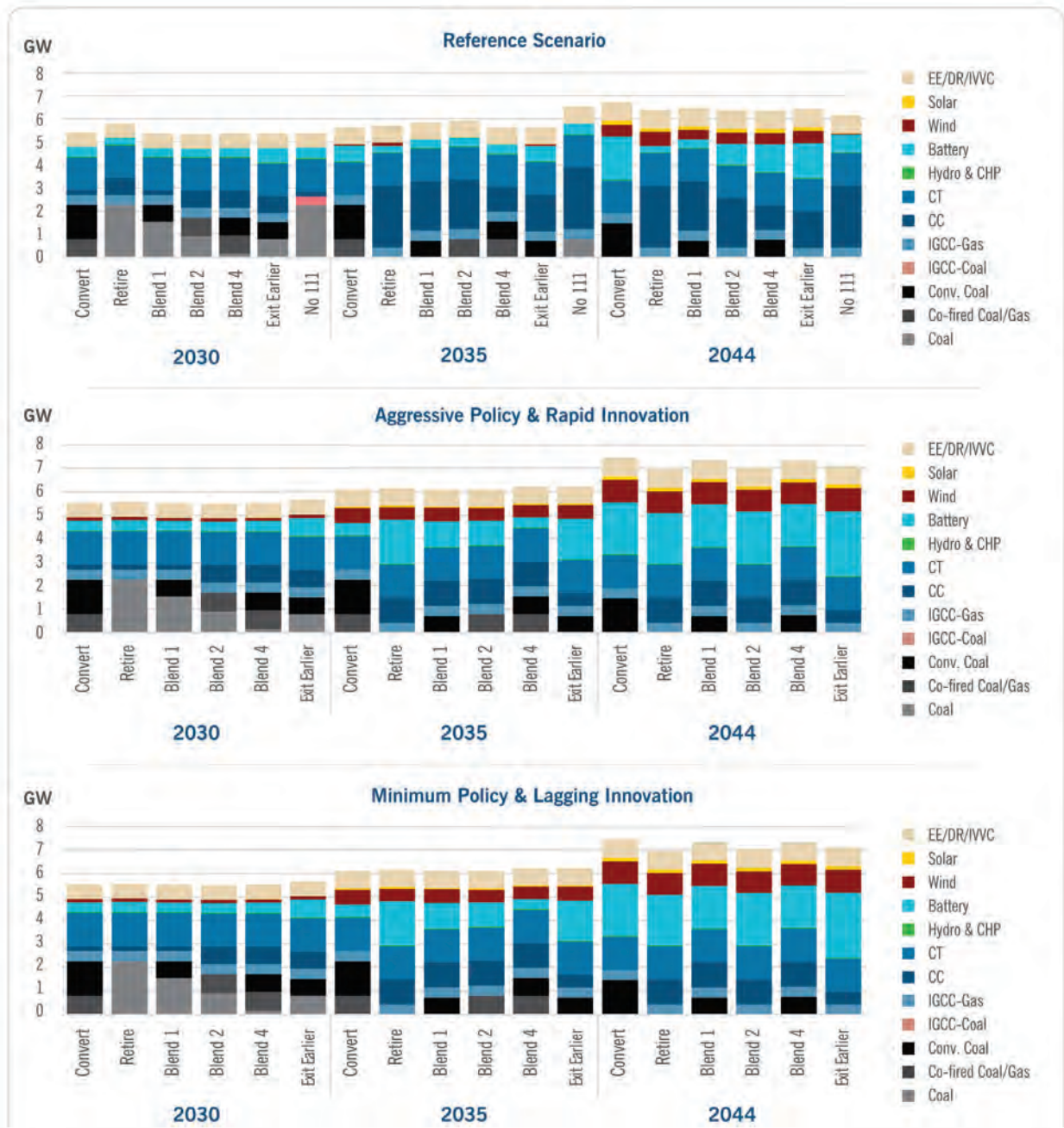
Figure 4-6: Firm Winter Capacity (GW, Beginning-of-Year Basis)
