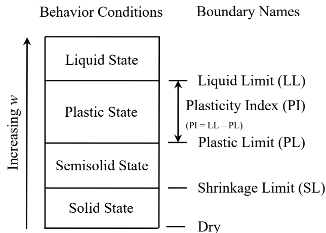
Figure 5.2 Consistency of soils as indicated by Atterberg limits
