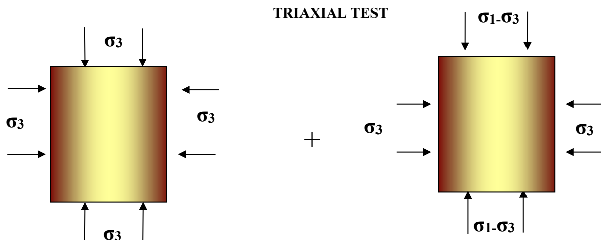
(a) Stress Conditions in a Typical Triaxial Test
