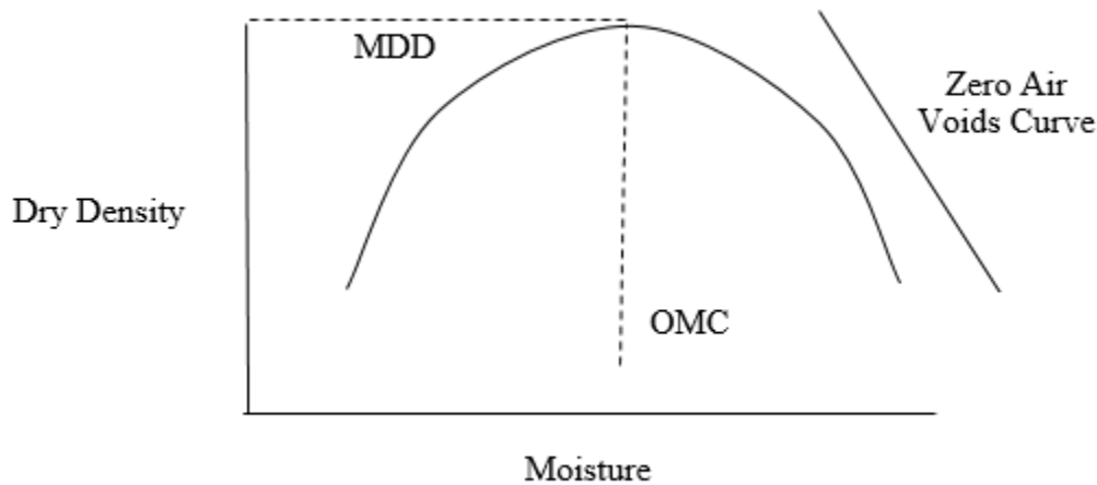
Figure 5.3 Standard Proctor compaction curve. Zero air voids curve represents 100% saturation.
