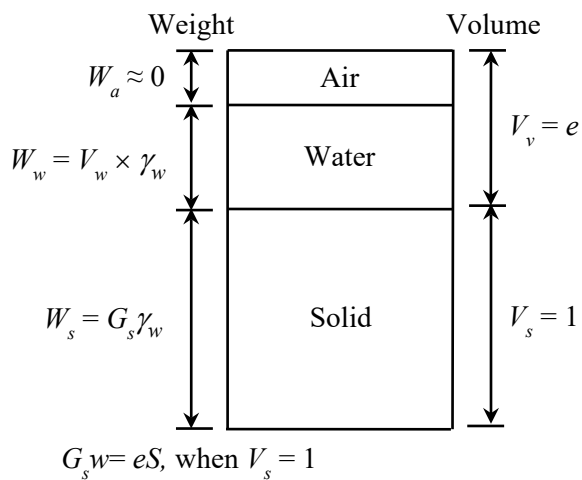
(b) Unsaturated soil; V_s = 1 , three-phase diagram
