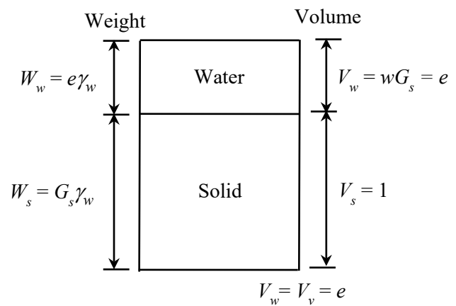
(c) Weight-volume relationships, two-phase diagram
