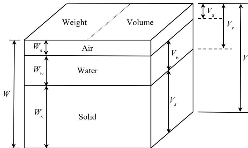
(a) Components of soils
