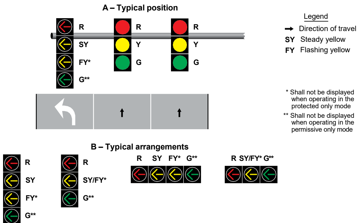
Figure 4F-7. Typical Position and Arrangements of Separate Signal Faces with Flashing Yellow Arrow for Protected/Permmissive Mode and Variable Mode Left Turns
