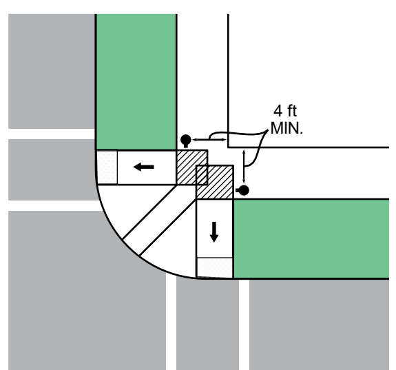
D – Perpendicular curb ramps with continuous surface between ramps
