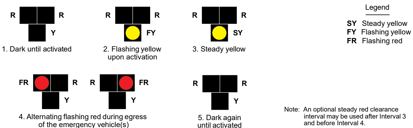
Figure 4N-1. Sequence for an Emergency-Vehicle Hybrid Beacon
