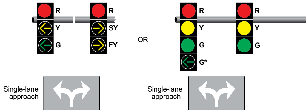
Figure 4F-15. Signal Indications for Approaches with a Combined Left-Turn/Right-Turn Lane and No Through Movement (Sheet 2 of 3)
