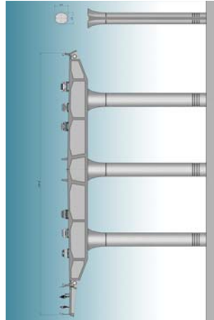
Bridge Concrete Box - Section
