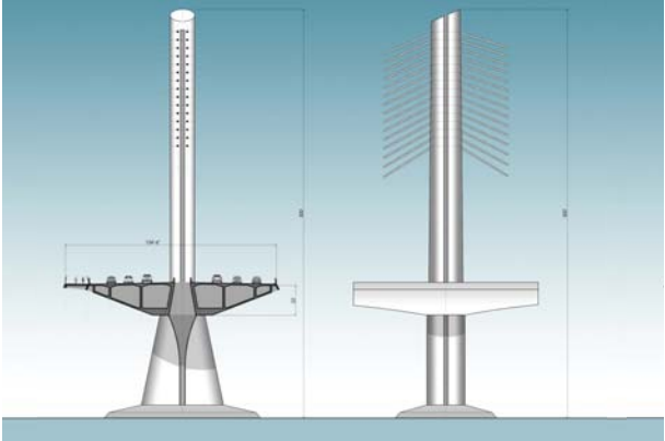
Bridge Tower - Section / Elevation
