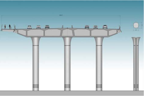
Single Concrete Box - Section
