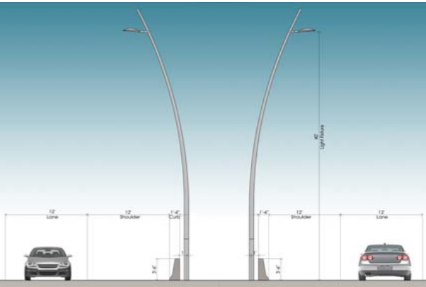
Luminaire Elevation
