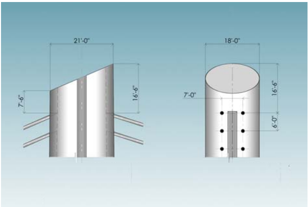
Bridge Tower - Details
