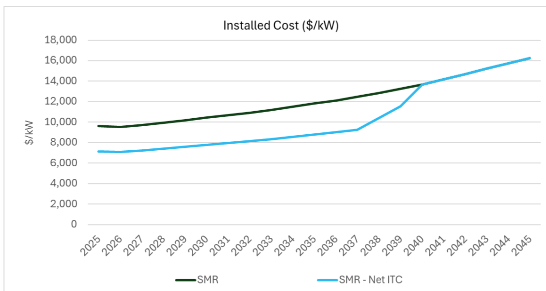
Figure 28. SMR Installed Costs
