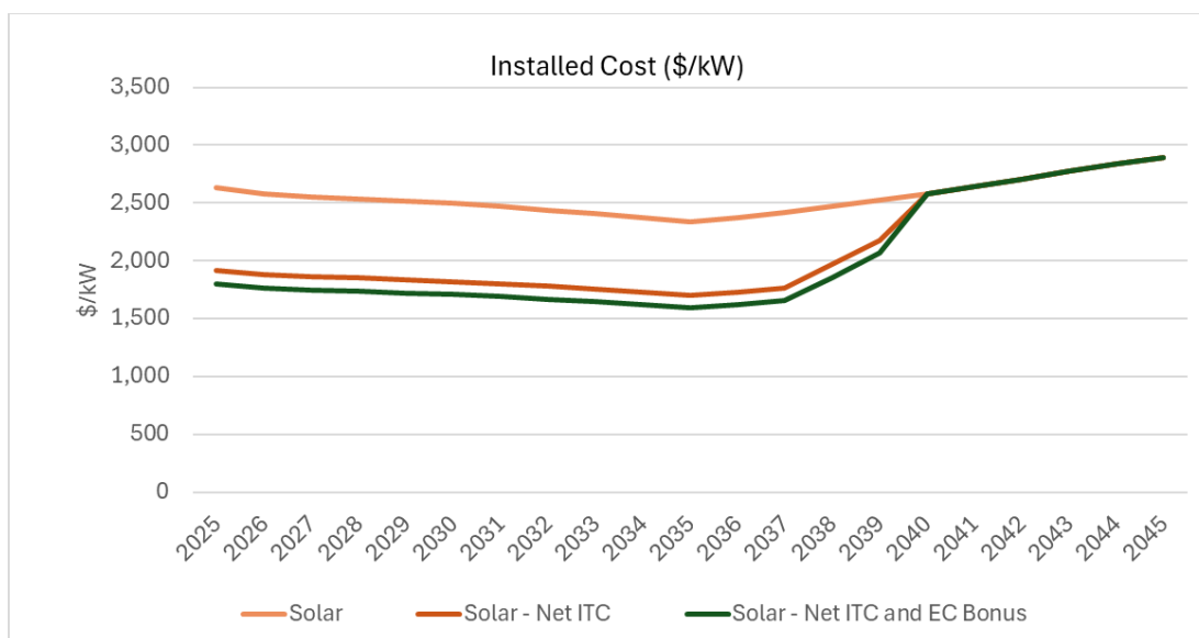
Figure 33. Solar Installed Costs
