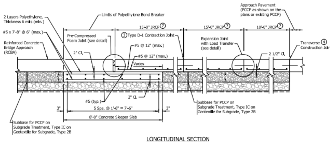
Figure 7-7 Terminal Joint
