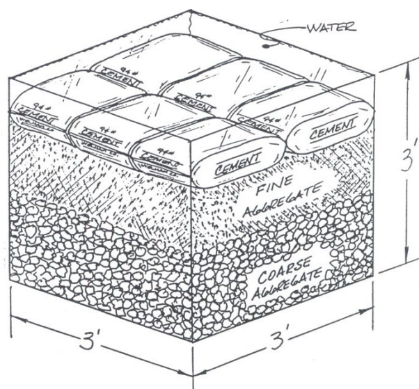
Figure 3-1 Concrete Materials
