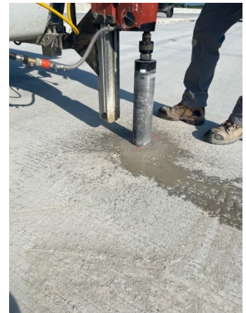
Figure 8-2 Concrete Coring
