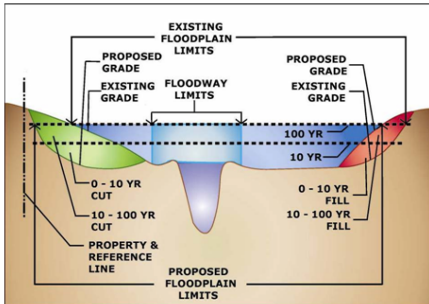
Figure 11-4 – Example Cross Section D-D
