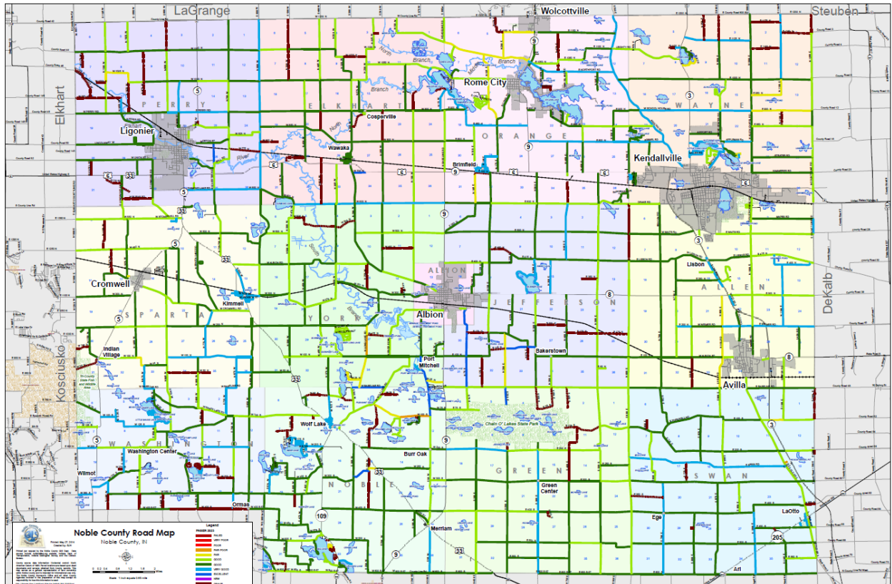
Figure 11 - Road Rating 2023
