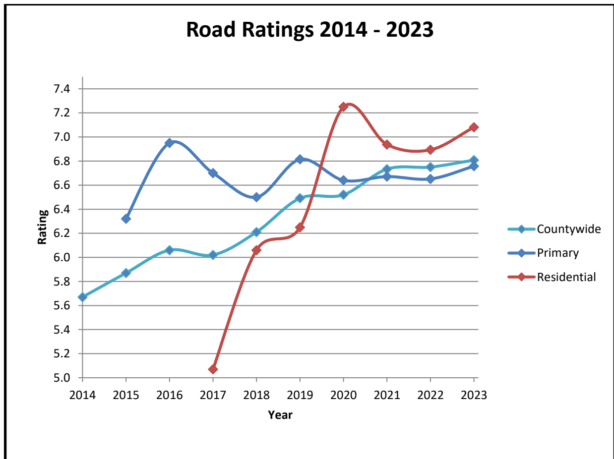
Figure 10 - Road Rating 2014 - 2023
