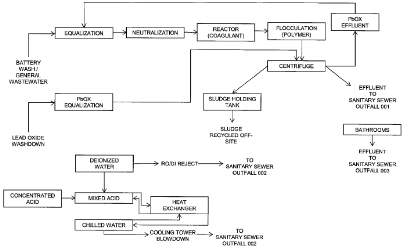
Figure 1: Flow Diagram
