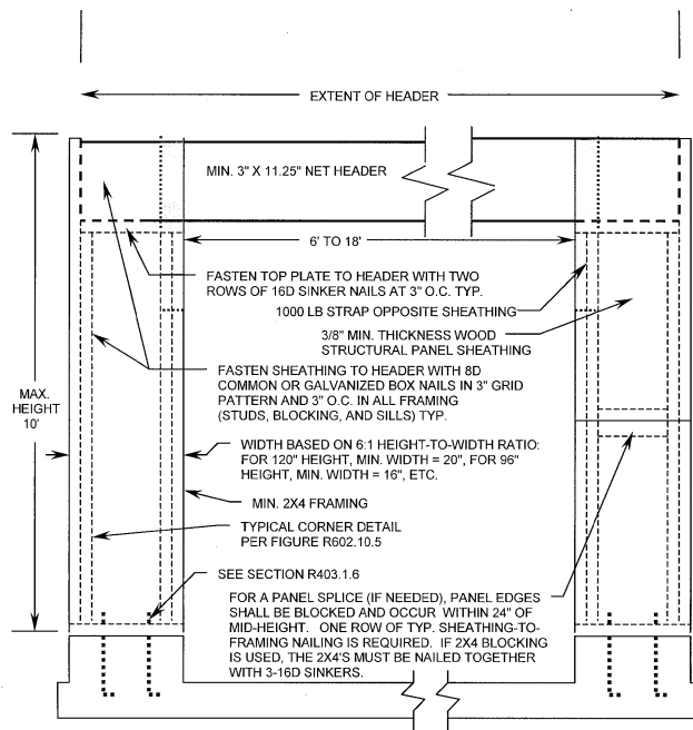
FIGURE R602.10.5(2)
