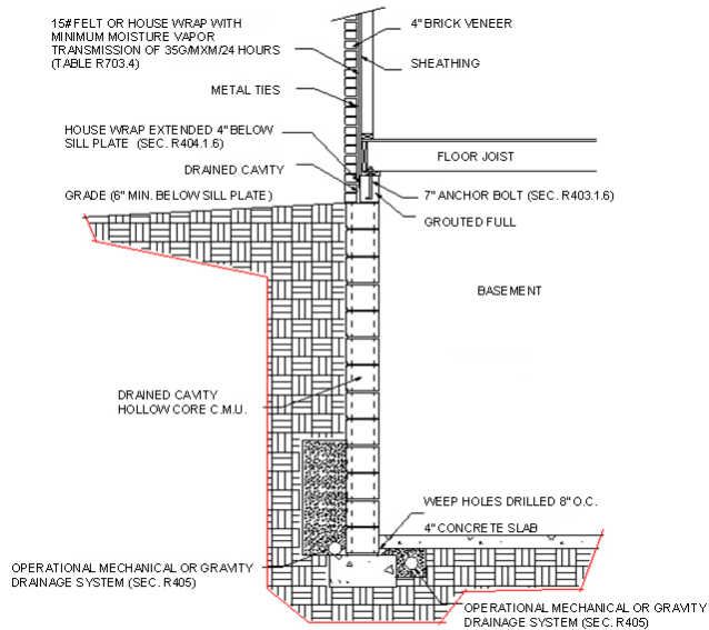
FIGURE R703.7.6(2)
