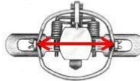
Figure 2 Inside distance between the trap's hinge posts.
