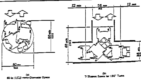
Fig. 3 Wheelchair Turning Space
