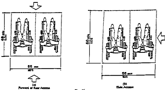
Space Requirements for Wheelchair Seating Spaces in Series
