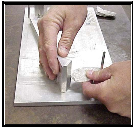
Figure 1 Checking Elongation
