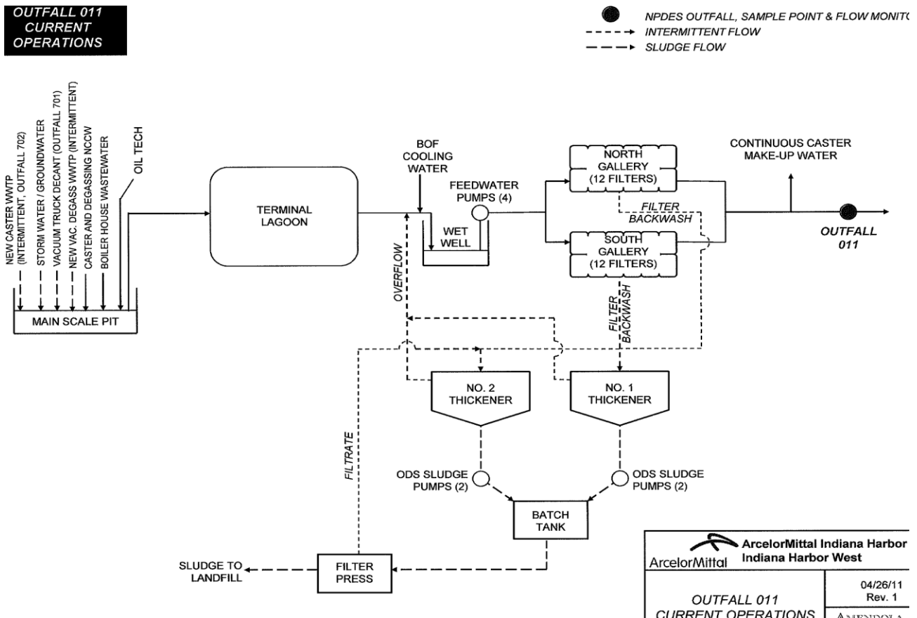
Figure 6: Flow Diagram of Outfall 011
