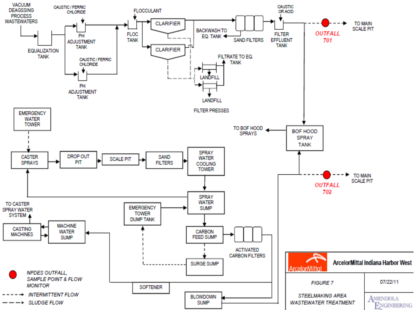
Figure 7: Flow Diagram of Internal Outfalls 701 and 702
