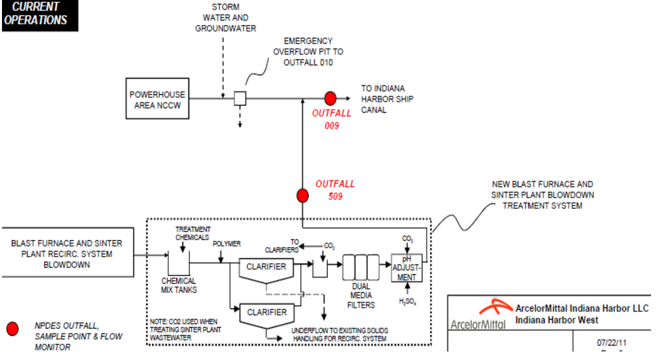
Figure 4: Current Operations at Outfall 009
