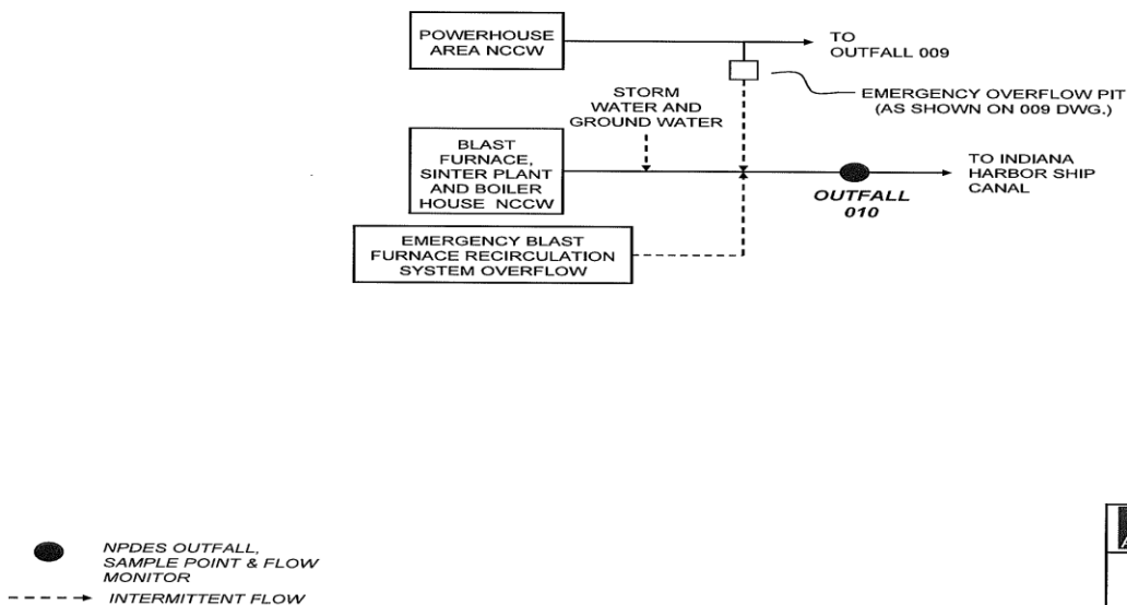
Figure 5: Flow Diagram of Outfall 010
