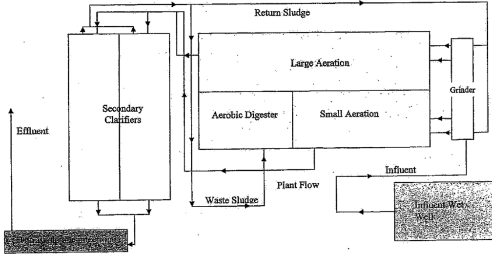
Maconaquah School Corporation Plant Flow Schematic
