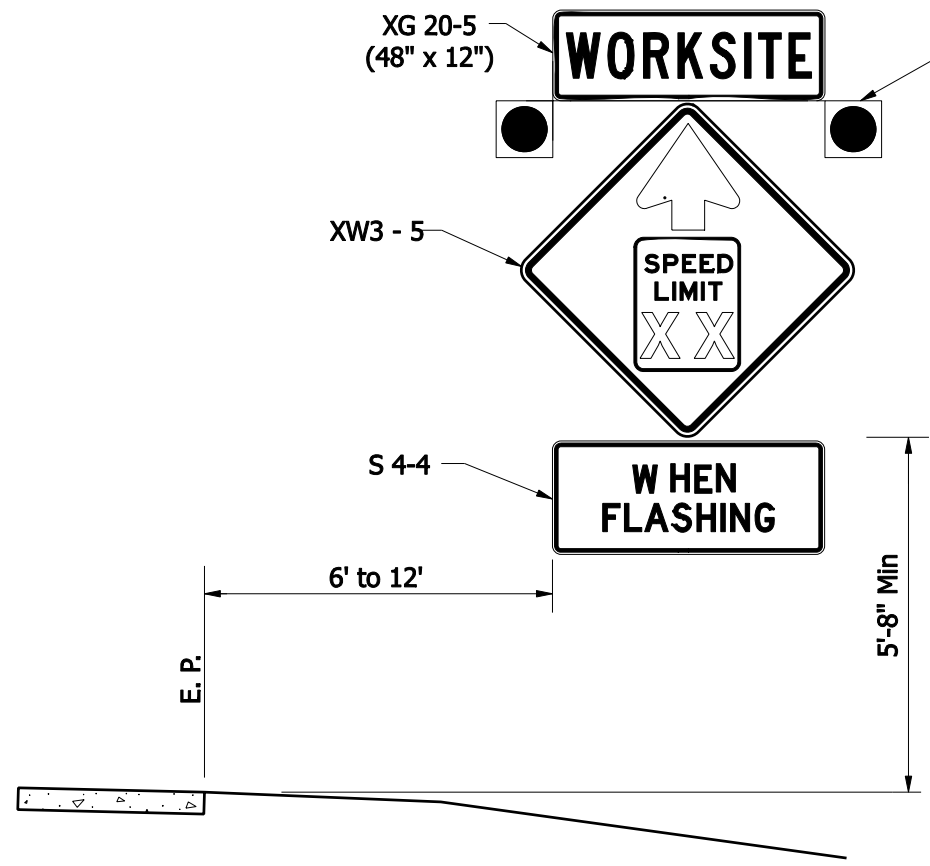
Reduced Speed Advance Warning Sign Assembly
