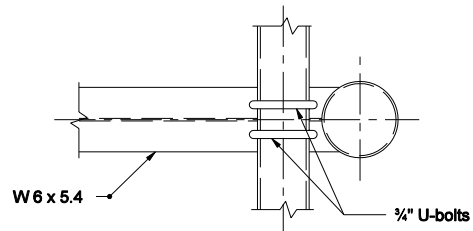
LOWER CHORD CONNECTION DETAIL
