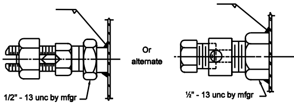
GROUNDING CONNECTION
