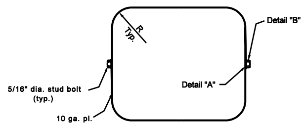
SKIRT DETAIL
