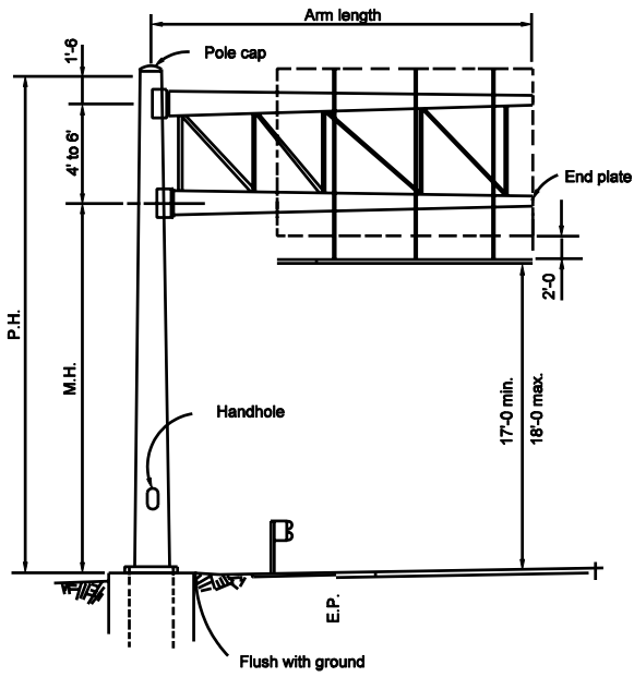
CANTILEVER (DOUBLE MASTARM)
