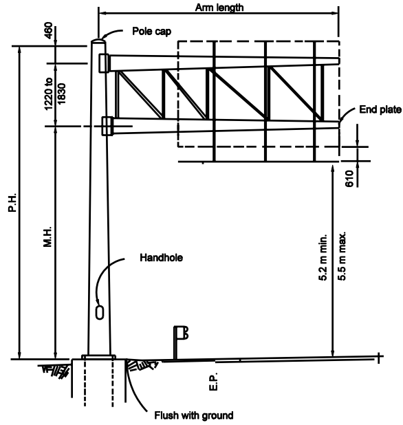
CANTILEVER (DOUBLE MASTARM)
