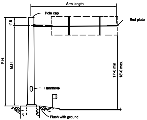
CANTILEVER (SINGLE MASTARM)
