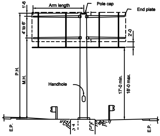
OVERHEAD BALANCED CANTILEVERS
