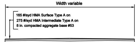
TYPICAL SECTION
