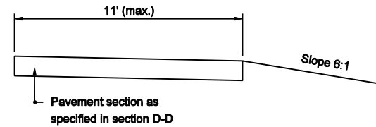
SECTION E-E
