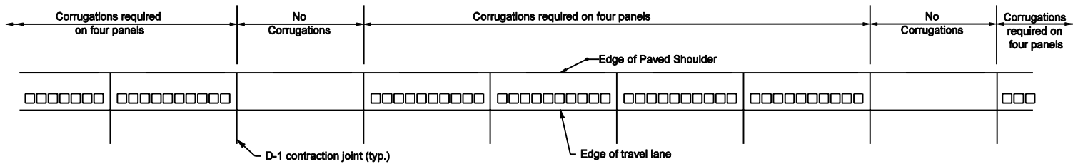
INTERMITTENT INSTALLATION DETAIL
