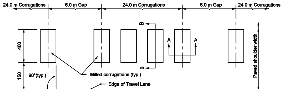
INTERMITTENT INSTALLATION PLAN VIEW
