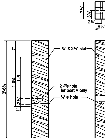
SIDE FRONT BCT TIMBER POST
