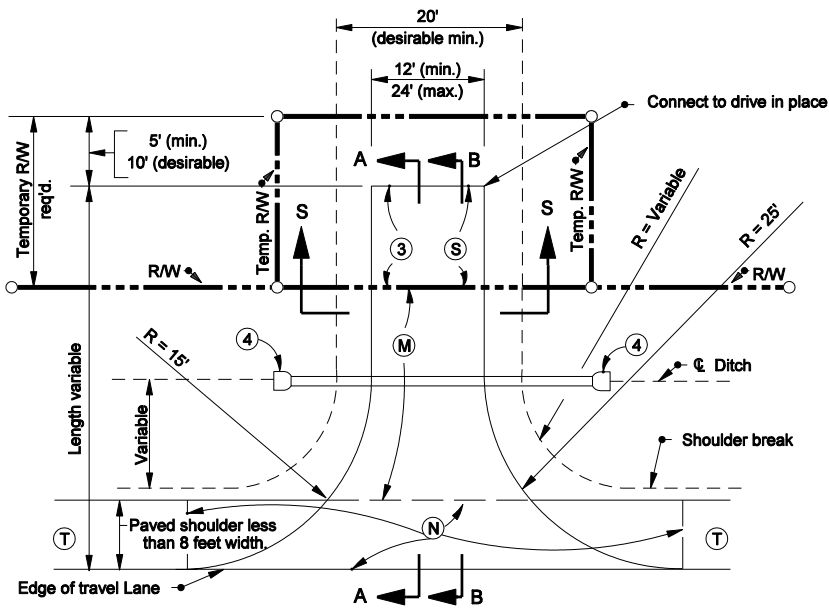
PLAN VIEW (PAVED SHOULDER LESS THAN 8 FEET IN WIDTH OR UNPAVED SHOULDER)
