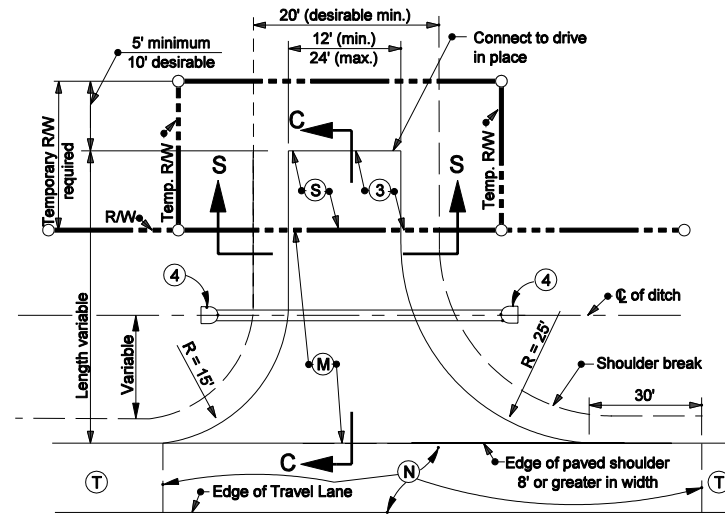
PLAN VIEW (PAVED SHOULDER 8 FEET OR GREATER IN WIDTH)
