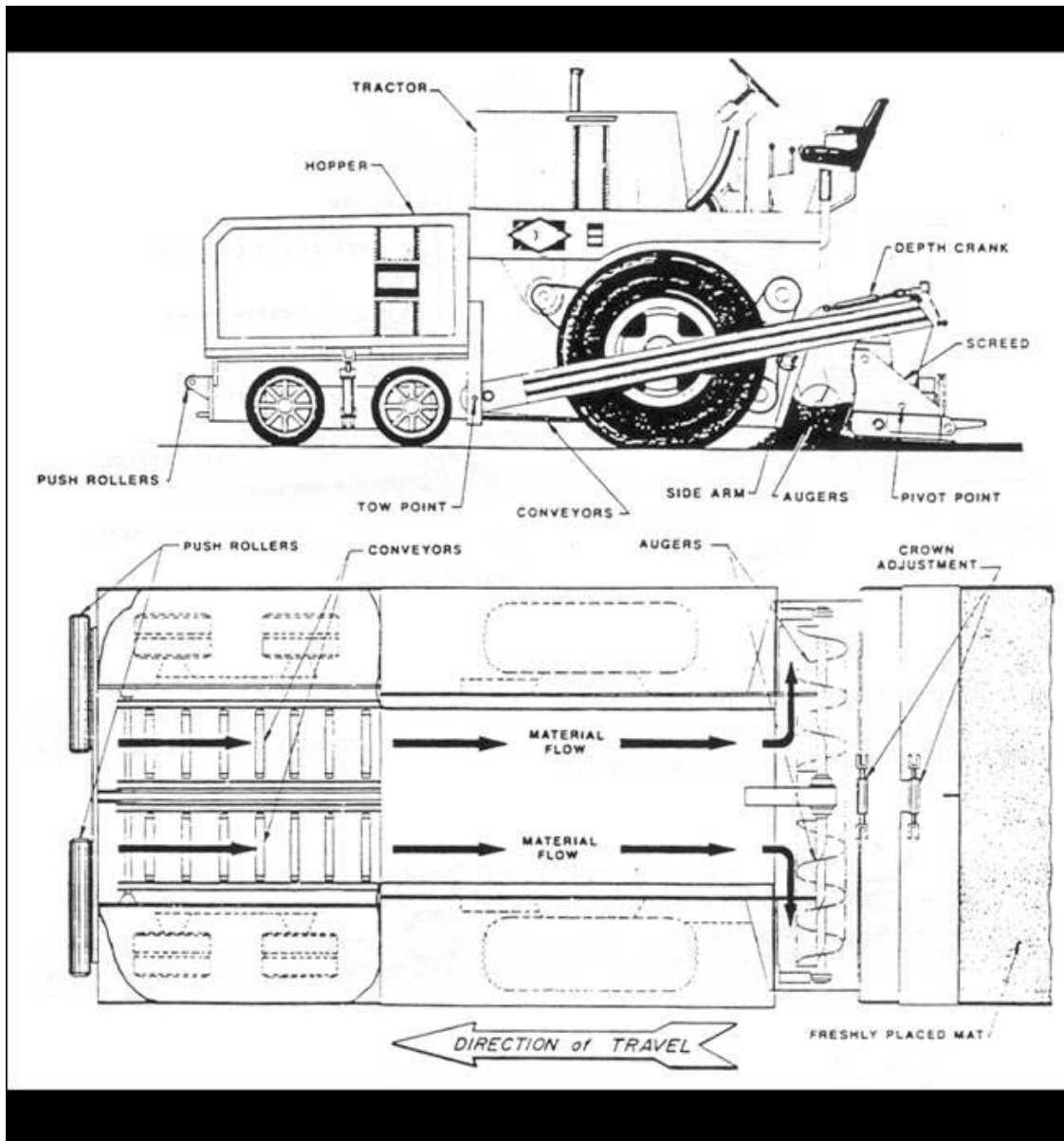
Figure 13.24-3 Asphalt Paver
