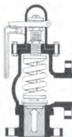
RELIEF VALVE
