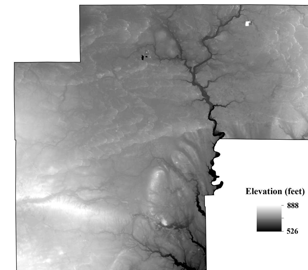
Digital Elevation Model of White County, IN
