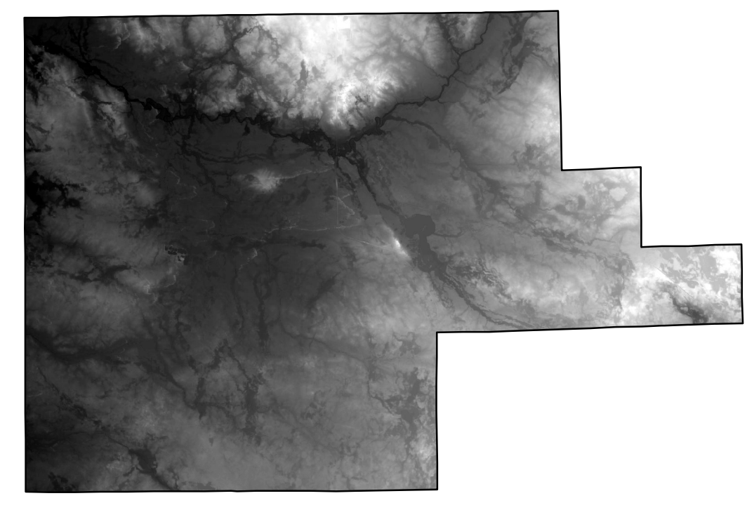
Digital Elevation Model of Fulton County, Indiana
