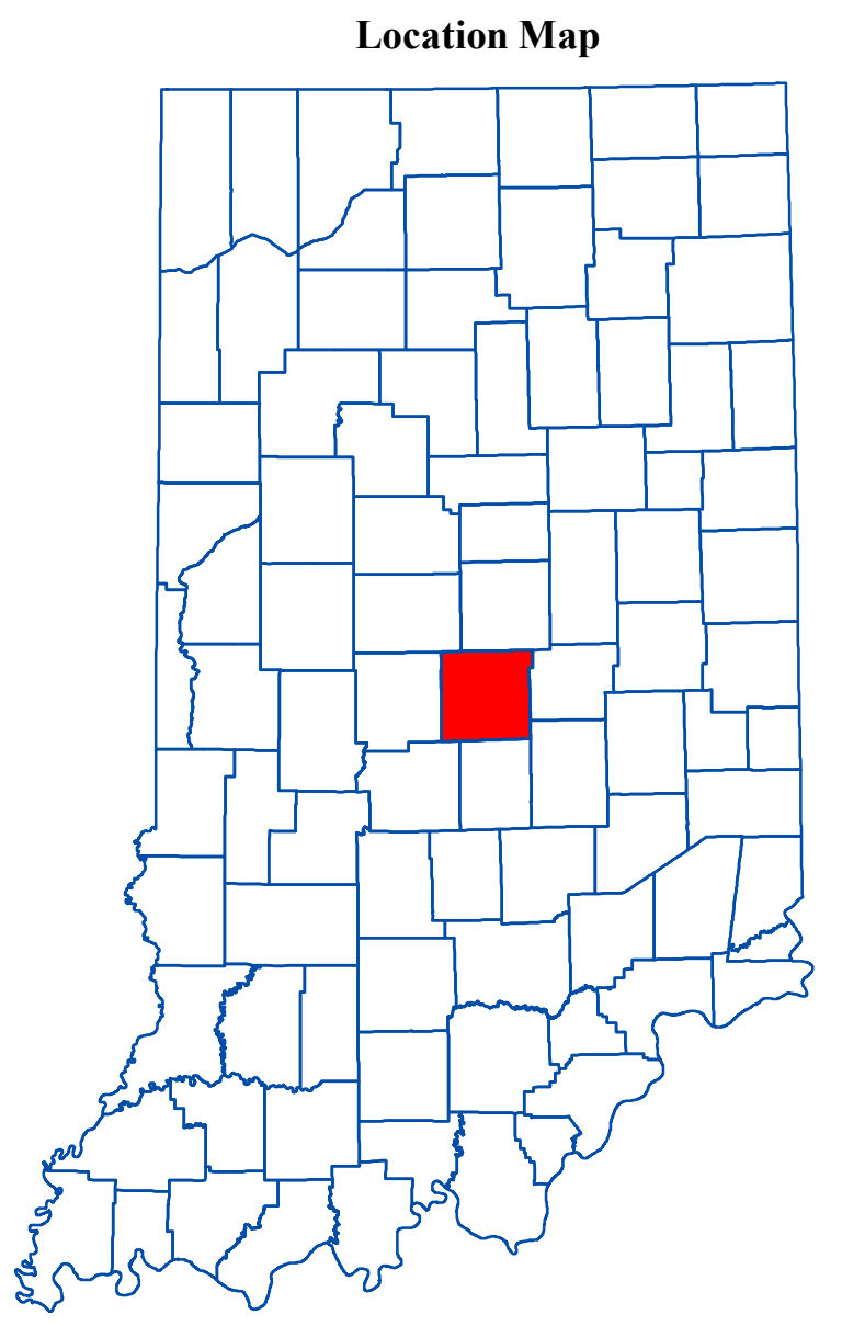
Digital Elevation Model of Marion County, Indiana
