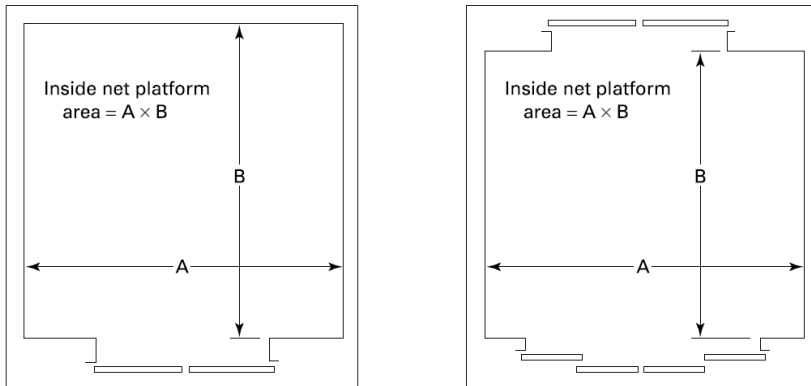
Figure 3.7.1 Inside Net Platform Areas for Passenger Elevators
