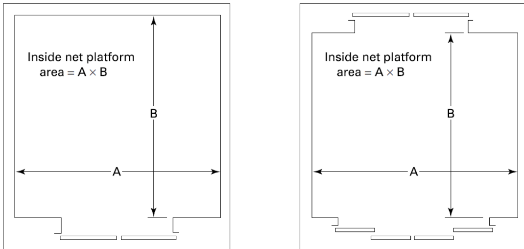
Figure 3.7.1 Inside Net Platform Areas for Passenger Elevators
