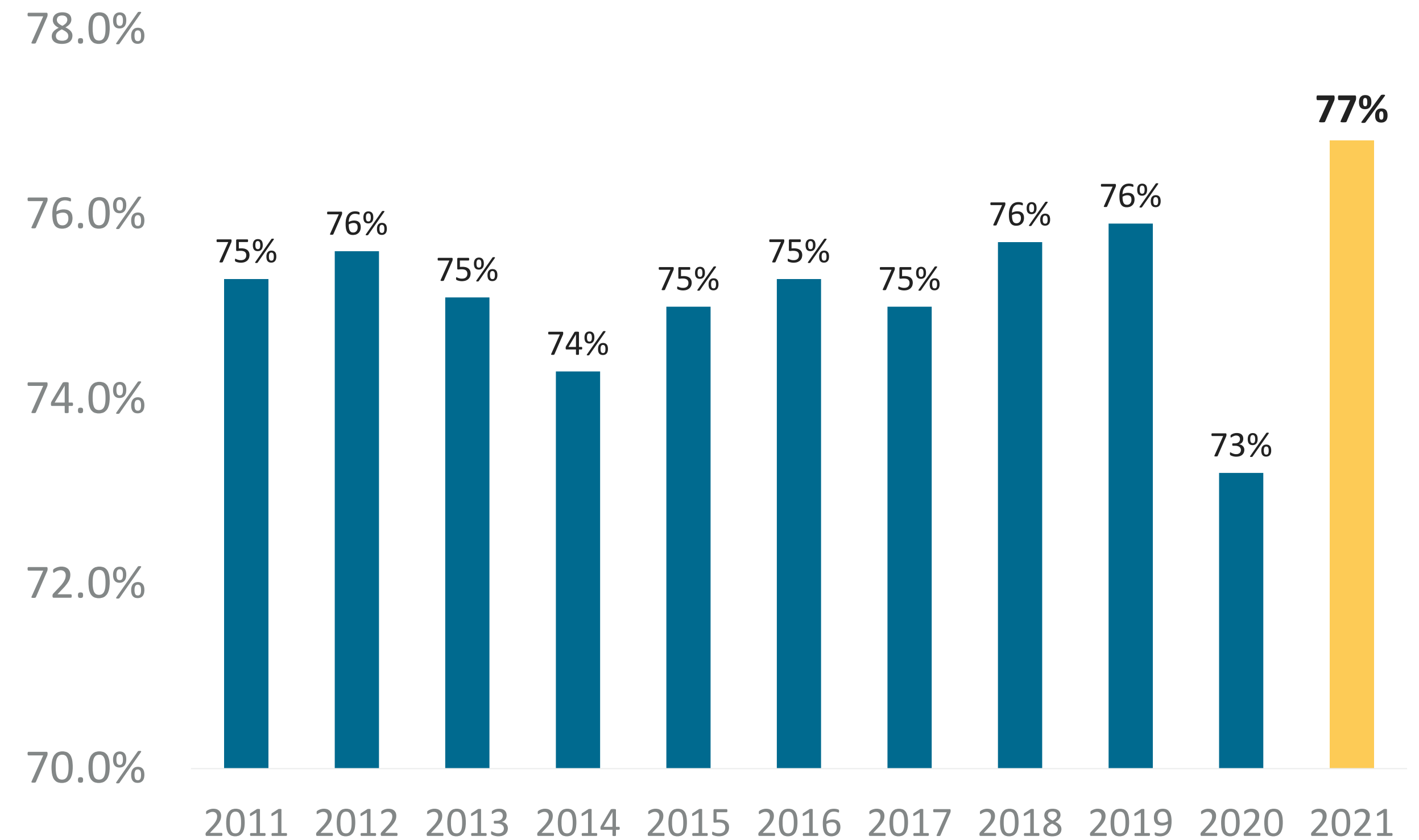
Persistence Rate by IN College Going Cohort
