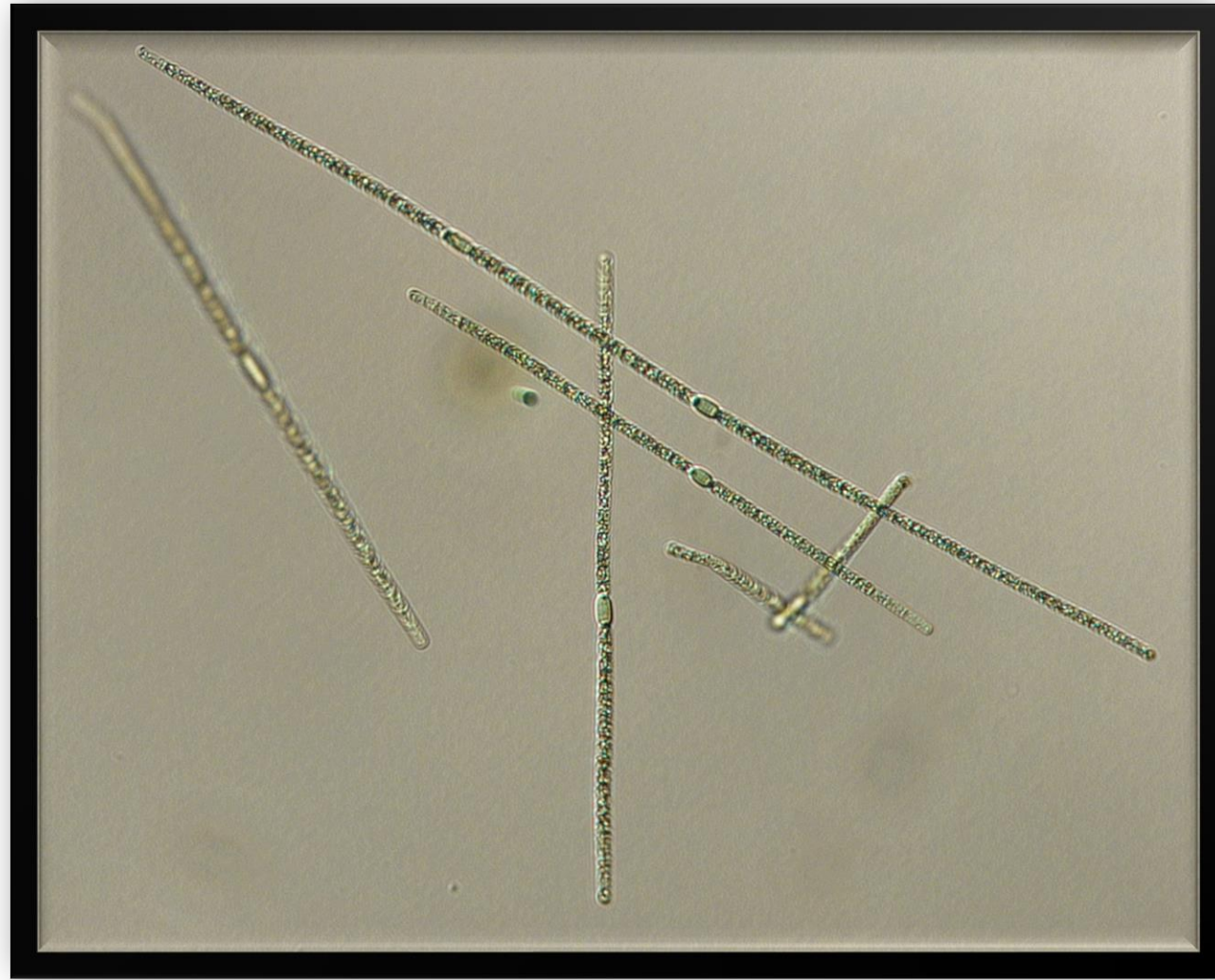
Saxitoxin
