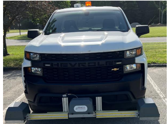
Figure 8-1 Inertial Profiler (attached to bumper)
