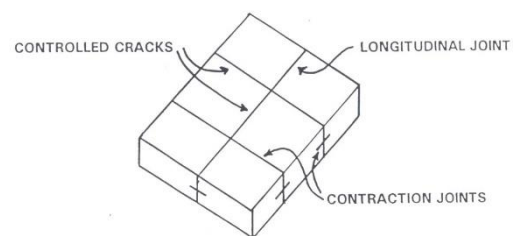
Figure 1-1 Plain Jointed Concrete Pavement
