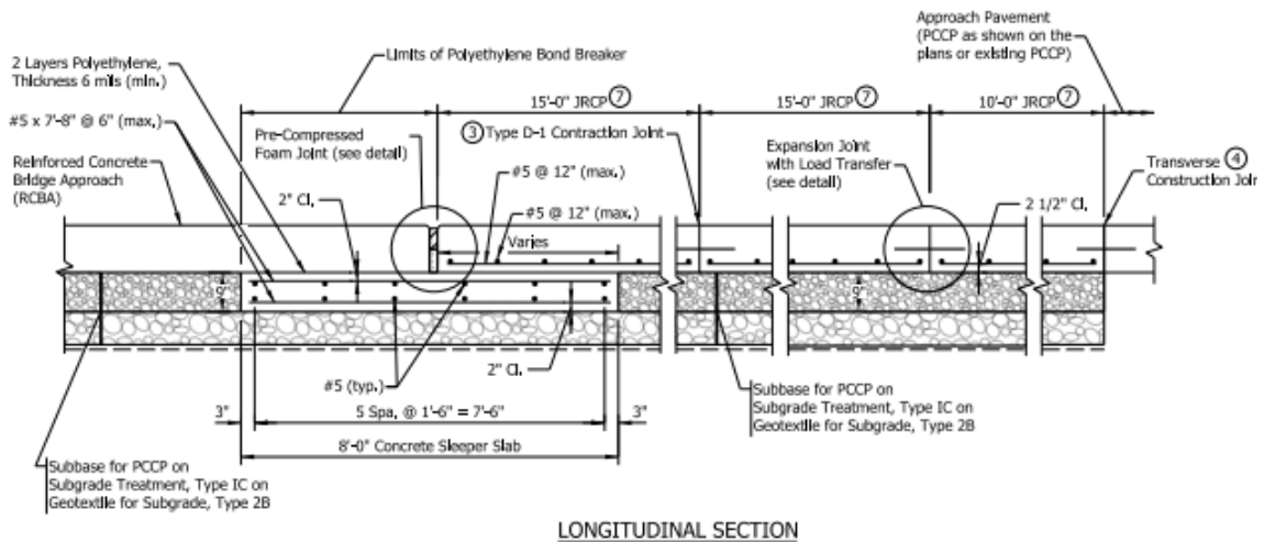
Figure 7-7 Terminal Joint
