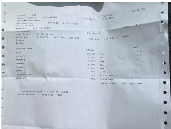
Figure 6-4 Concrete Ticket, paper form
